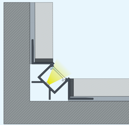
EN Installation instruction for profile VIGO with a BASIC cover.
