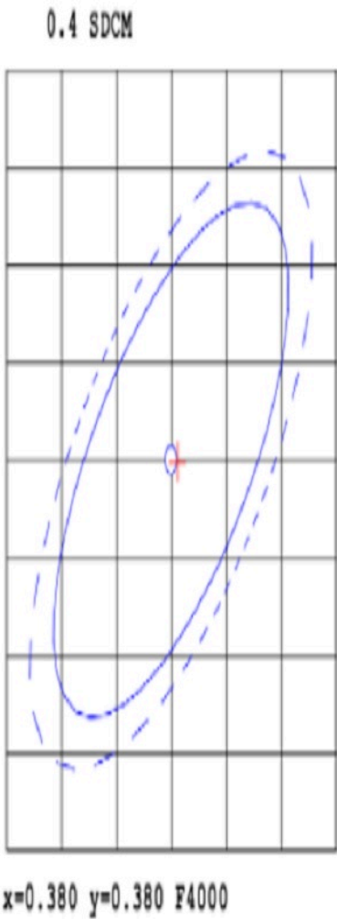
CIE1931 Chromaticity Diagram
